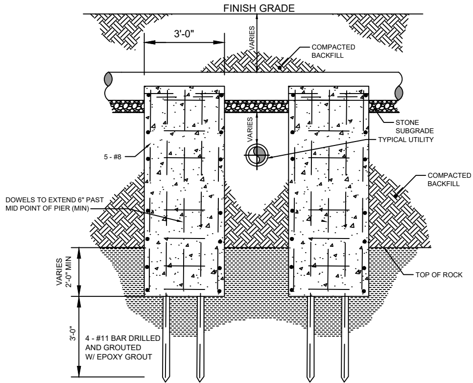
SIDE ELEVATION NOT TO SCALE
