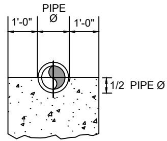
BELOW GRADE STORM SEWER CROSSING NOT TO SCALE
